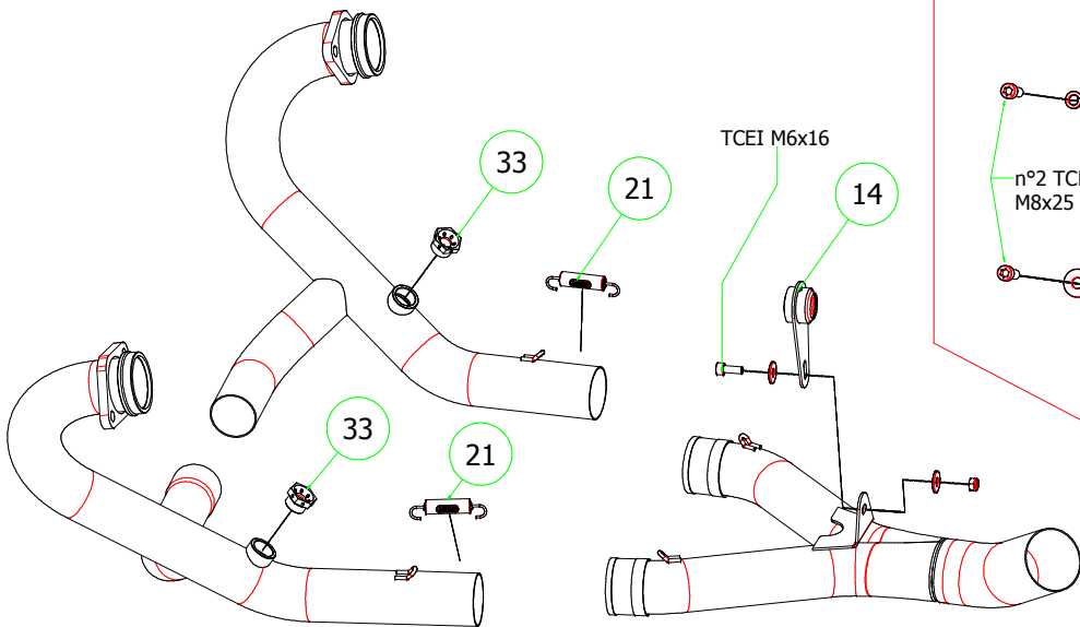
71426MI Mid-Pipe (Arrow Collectors)
