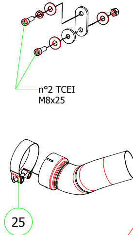
71466MI Mid-Pipe (Arrow + Original)
