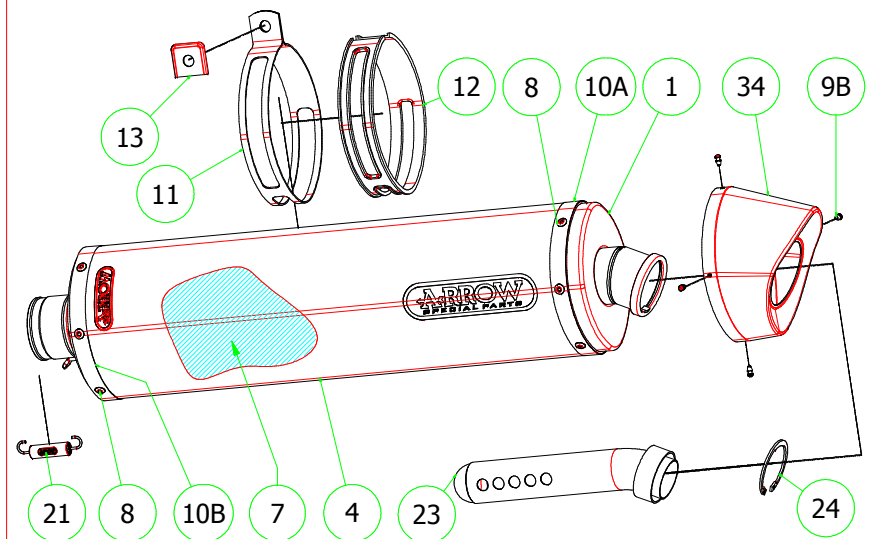
71689PK Homologated Titanium-Carbon 71689AK Homologated Aluminium-Carbon 71689AKN Homologated Aluminium-Carbon (Dark Line)
