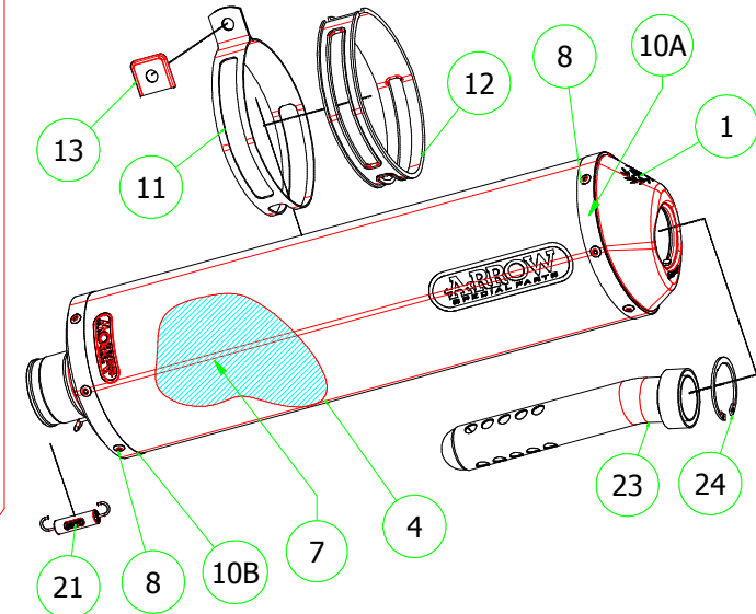
71689PK Homologated Titanium-Carbon 71689AK Homologated Aluminium-Carbon 71689AKN Homologated Aluminium-Carbon (Dark Line)
