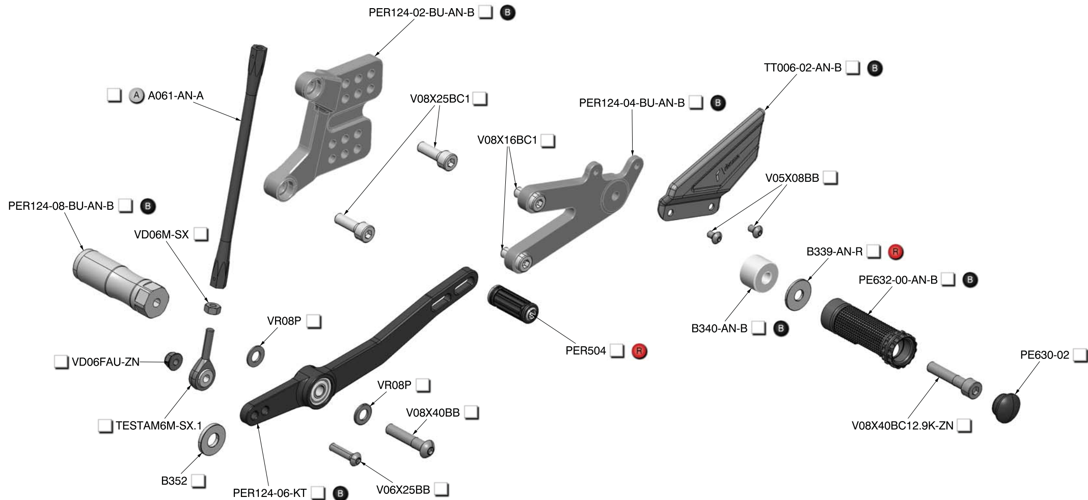
PER124-SX (Comandi arretrati lato SX completi) B (Complete LH rear set control kit)
