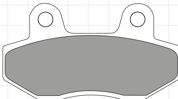
ODP020 76.4 x 42.1 x 7.1mm
