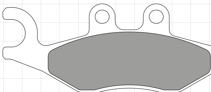
ODP018 97 x 41 x 9.0mm 77 x 41 x 9.0mm
