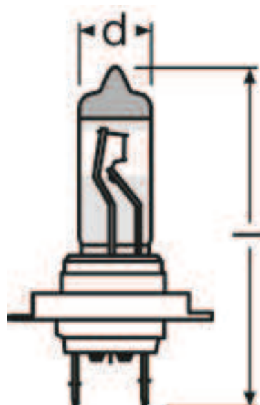
Product line drawing 64210NRP
