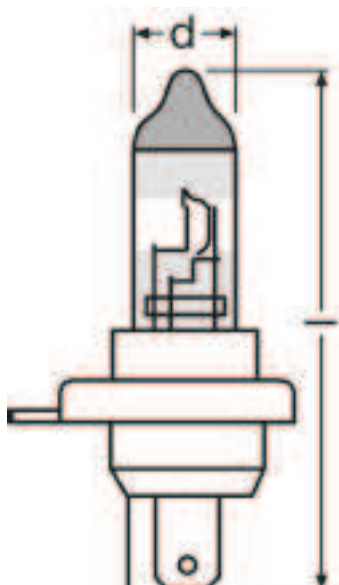
Product line drawing 64193NRP
