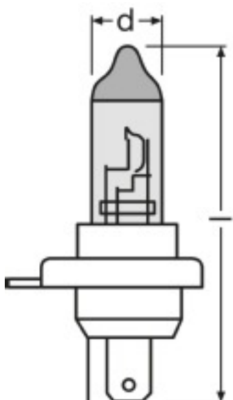
Product line drawing 64193XR
