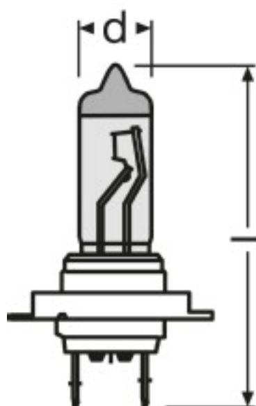
Product line drawing 64210XR
